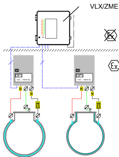
VLX 330/A-EX with VLX/ZME on several underground storage tanks.
