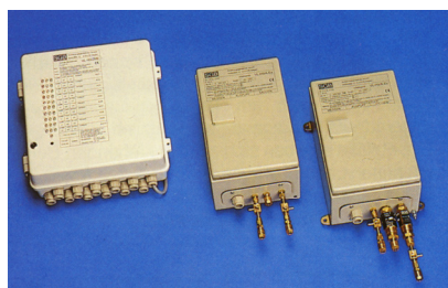
Leak detector VLX../A-Ex with central indicating device VLX/ZME. Up to 10 leak detectors can be connected to the VLX/ZME.
